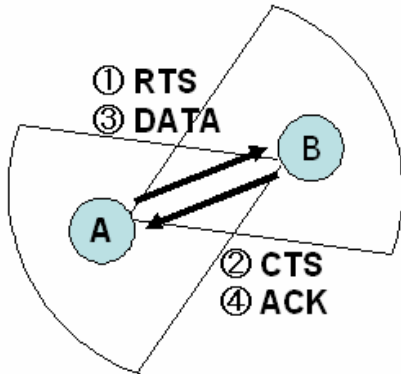
Figure 5 Data Transmission Using DVCS
