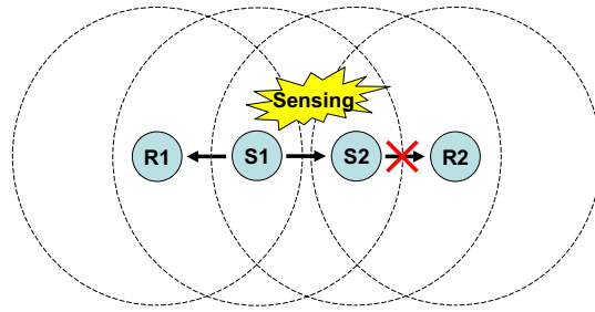
Figure 1 The Exposed Terminal Problem
