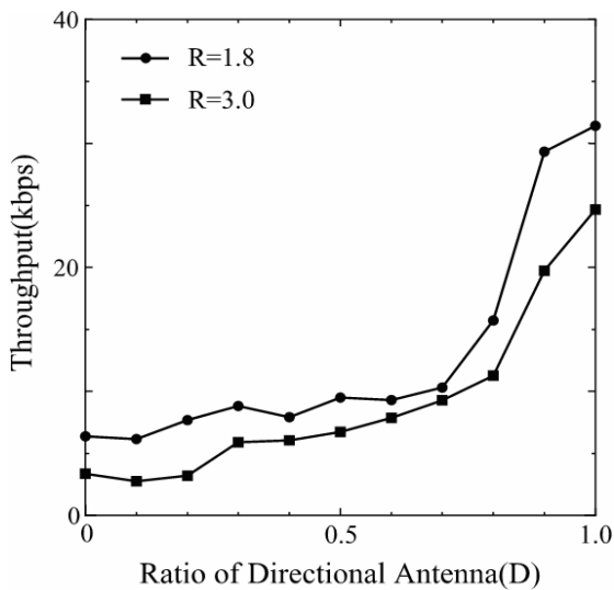
Figure 8 TCP Throughput Performance
