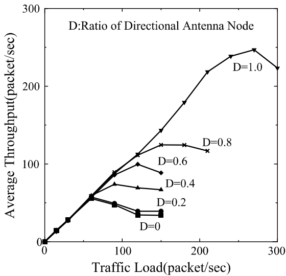
Figure 6 UDP Throughput Performance(R=1.8)
