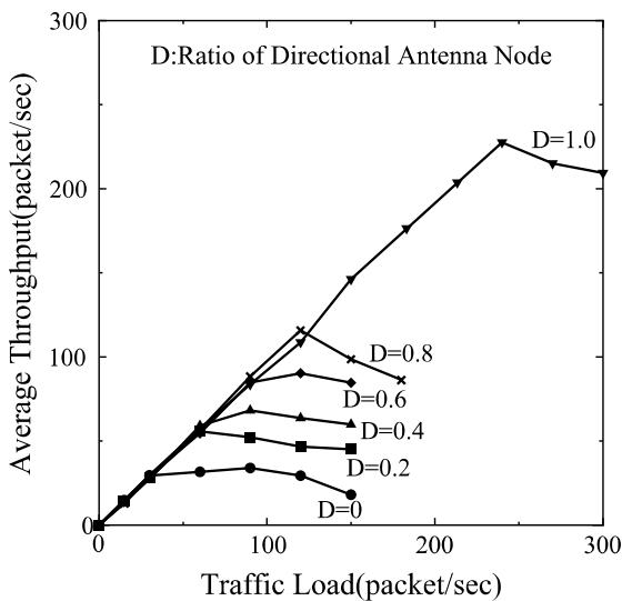
Figure 7 UDP Throughput Performance(R=3.0)
